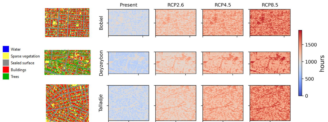
FIGURE 11 Number of lost working hours (LWH) per year for moderate activities for present (2001–2020) and future scenarios (2041–2060). Land use maps for the three districts depicted are added for clarity. A clear increase in LWH is visible in each scenario, almost doubling for the RCP8.5 scenario by 2041–2060. [Colour figure can be viewed at wileyonlinelibrary.com ]
