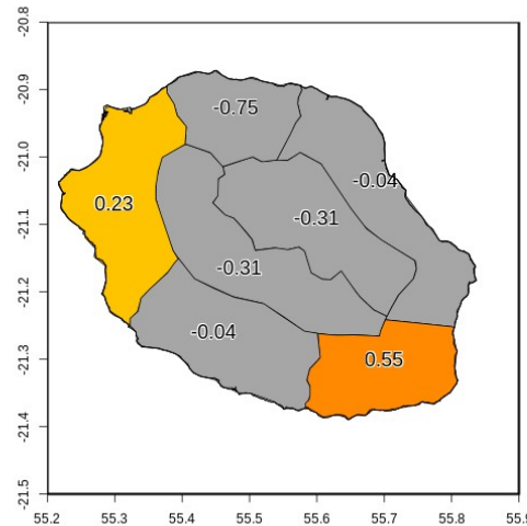
Score RPSS: RR_7ZONES NDJ-2020 It1
