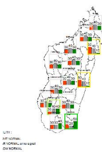
Rainfall Seasonal forecast - DJF 2020 - It 1
