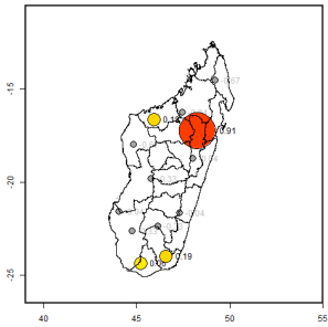
Forecast model: Mix - MixFcstRnd
