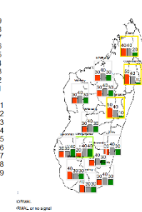
Rainfall Seasonal forecast - NDJ 2020 - It 2
