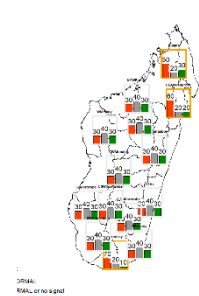
Rainfall Seasonal forecast - NDJ 2020 - It 1
