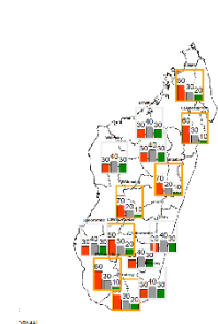
Rainfall Seasonal forecast - NDJ 2020 - It 3
