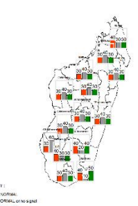
Rainfall Seasonal forecast - DJF 2020 - It 2
