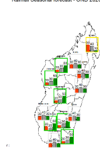
Rainfall Seasonal forecast - OND 2020 - It 3
