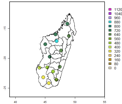
RR Avg.: NDJ
