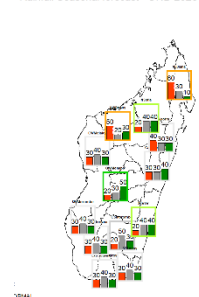
Rainfall Seasonal forecast - OND 2020 - It 2
